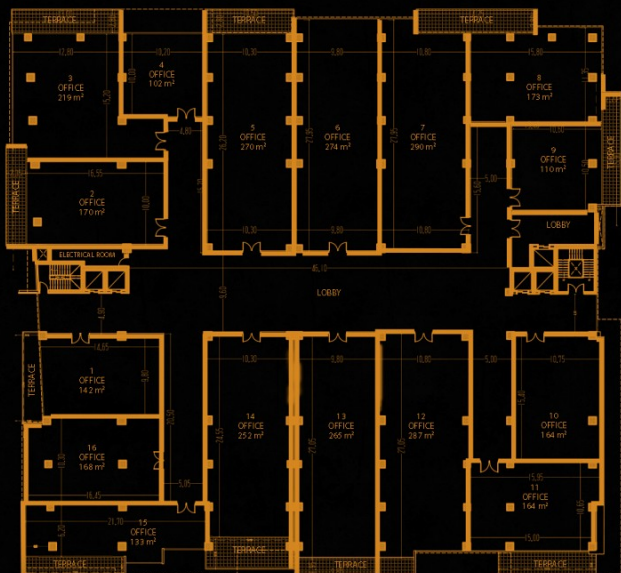
THIRD FLOOR PLAN AREA : 4142.3 PLOT 4/33
