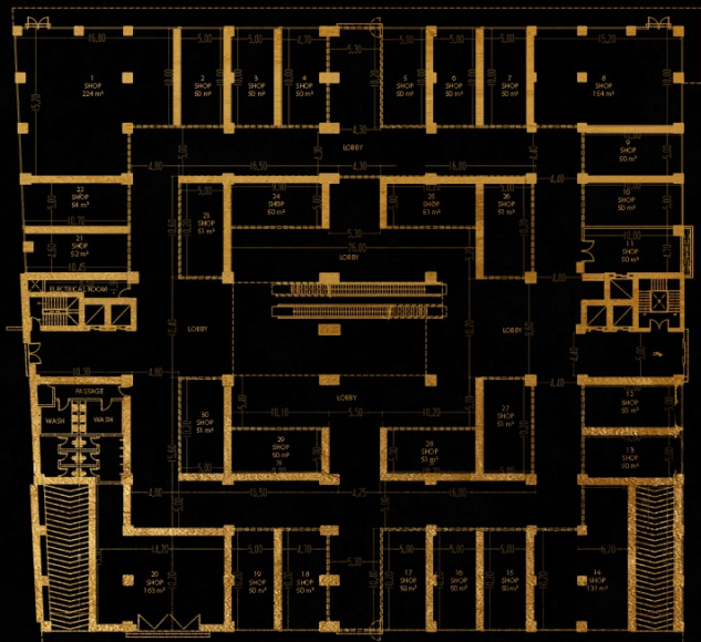
GROUND FLOOR PLAN AREA : 4204
